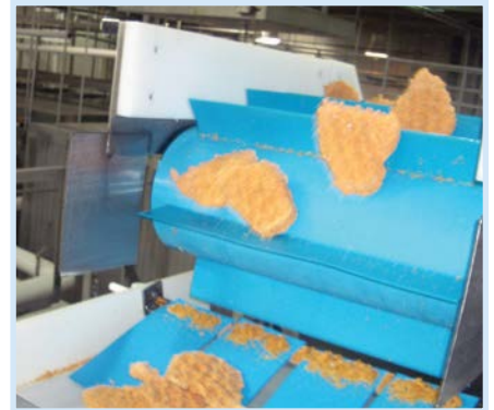
DualDrive™ on breaded chicken breast line
